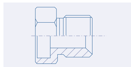
BSP Hexagon Male Welding Bosses 52.808.
