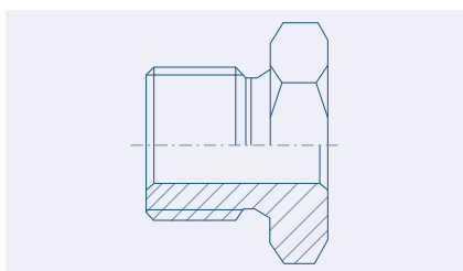
BSPP Male x BSP Fixed Female Adapter 52.5001.
