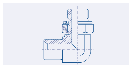
90° Elbow Adjustable BSPP Male 52.7009.
