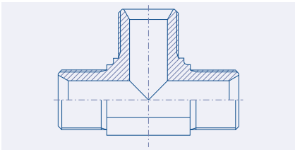
Union BSPP Male Tee 53.300.
