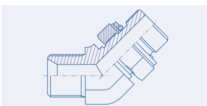
45° Elbow Adjustable BSPP Male 52.7008.
