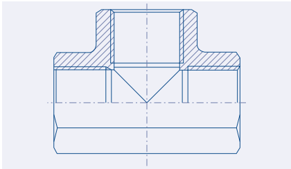
Fixed Female BSPP Tee 53.302.
