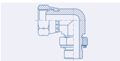
90° Elbow Adjustable BSPP Male x Female 52.7010.
