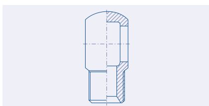
BSP Threaded Banjo Eye 52.800.
