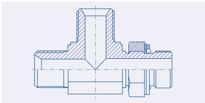
BSPP Male Adjustable Run Tee 52.7013.
