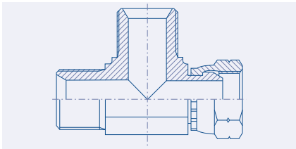
Swivel BSP Run Tee 53.4011.
