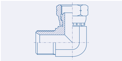
90° Elbow BSPP Male x Female 53.110.
