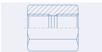
BSPP Female Union 52.3000.
