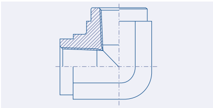
90° BSPP Elbow Fixed Female Union 53.120.
