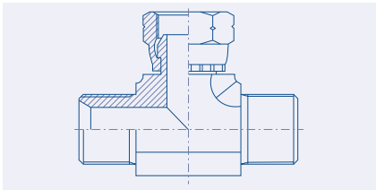
Swivel BSP Branch Tee 53.4012.
