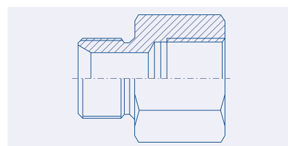
BSPP Male x BSP Fixed Female Adapter 52.5000.
