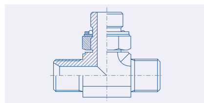
BSPP Male Adjustable Branch Tee 52.7012.
