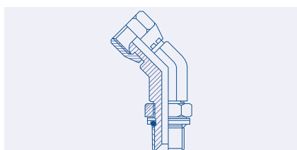
45° Elbow Adjustable BSPP Male x Female 52.7011.
