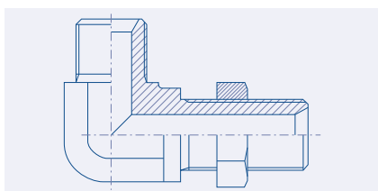
90° Elbow BSP Bulkhead Connector 52.5005.
