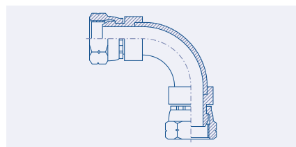
90° Elbow Swivel Female BSP
