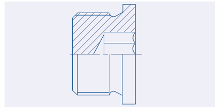
BSP Inner Hexagon Male Plug
