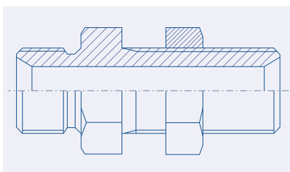
BSP Bulkhead Connector 52.5003.
